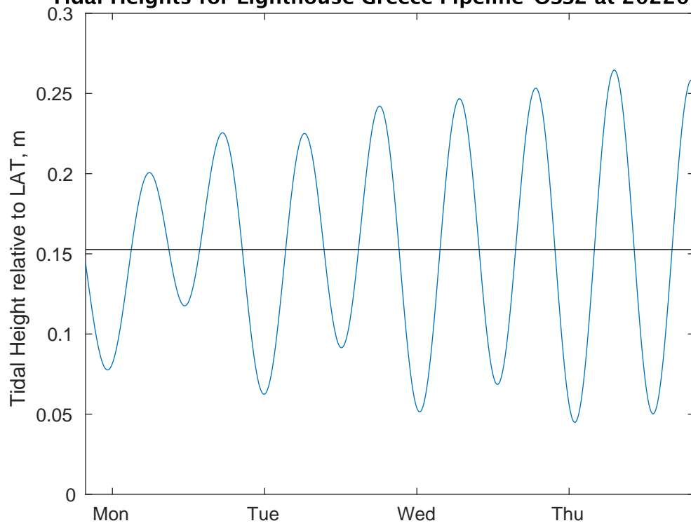
Tidal Heights for Lighthouse Greece Pipeline-OSS2 at 20220424
